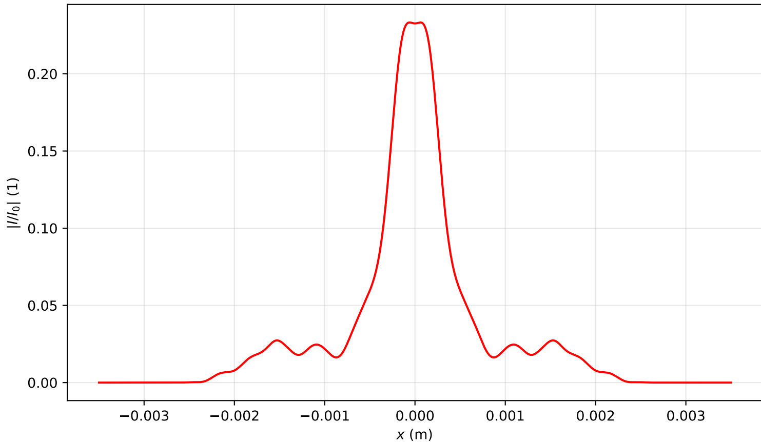
Intensity profile I(x, y = 0, z = 3.821)/I_0 , P_{in}=5.0P_{cr} , artificial time
